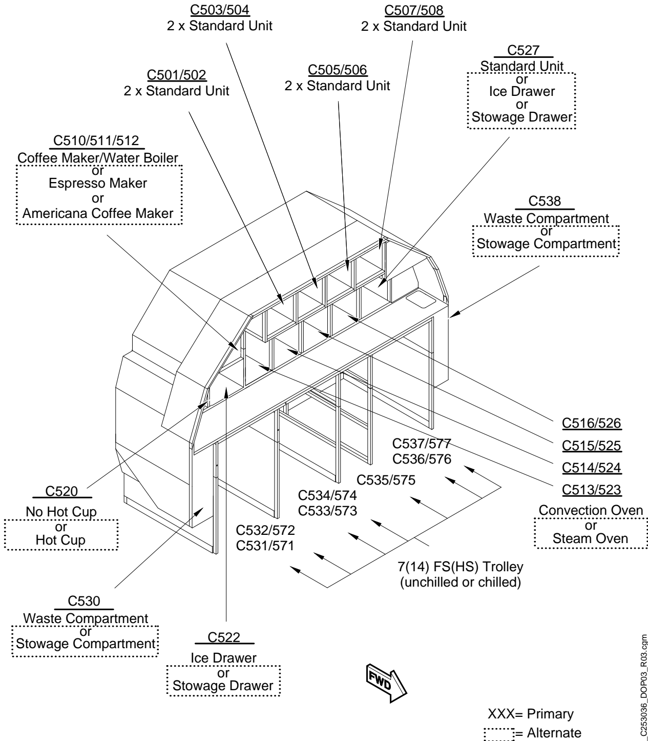
MODULAR GALLEY G5 - ACCESSORIES AND EQUIPMENT FIGURE 3
